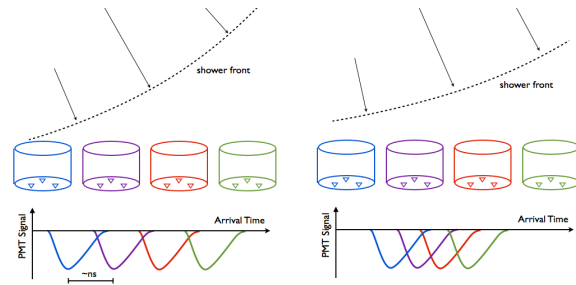
Figure 2: Diagram of two possible showers hitting 4 WCDs in the array. The relative arrival time is used to estimate the direction of the incoming gamma ray.
